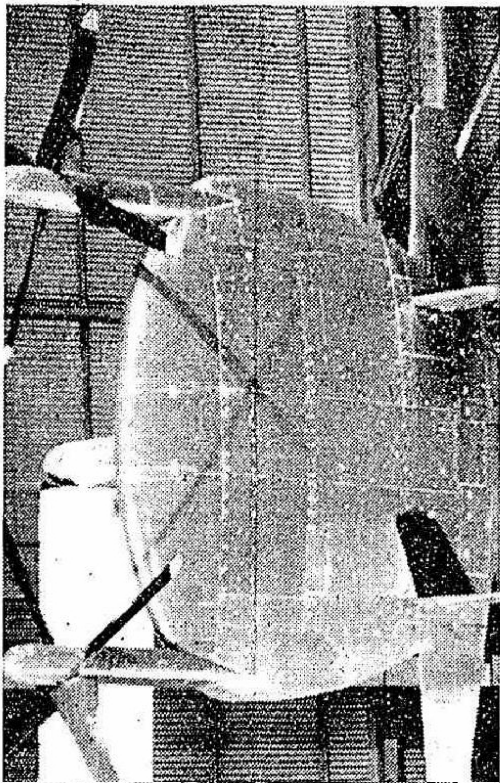
THE ORIGINAL flying saucer? This picture was published in America with an article that says there is competent evidence that flying saucers are real aircraft of revolutionary design, developed in the United States. This scale model, built in 1942, is mounted for wind tunnel tests at the laboratory of the National Advisory Committee for Aeronautics. It is
